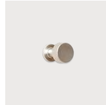
Angle Hook, Steel, Small Product no.: 3306 Material: Stainless Steel Finish: Matt Blasted Size: Ø: 2 cm, D: 3 cm
